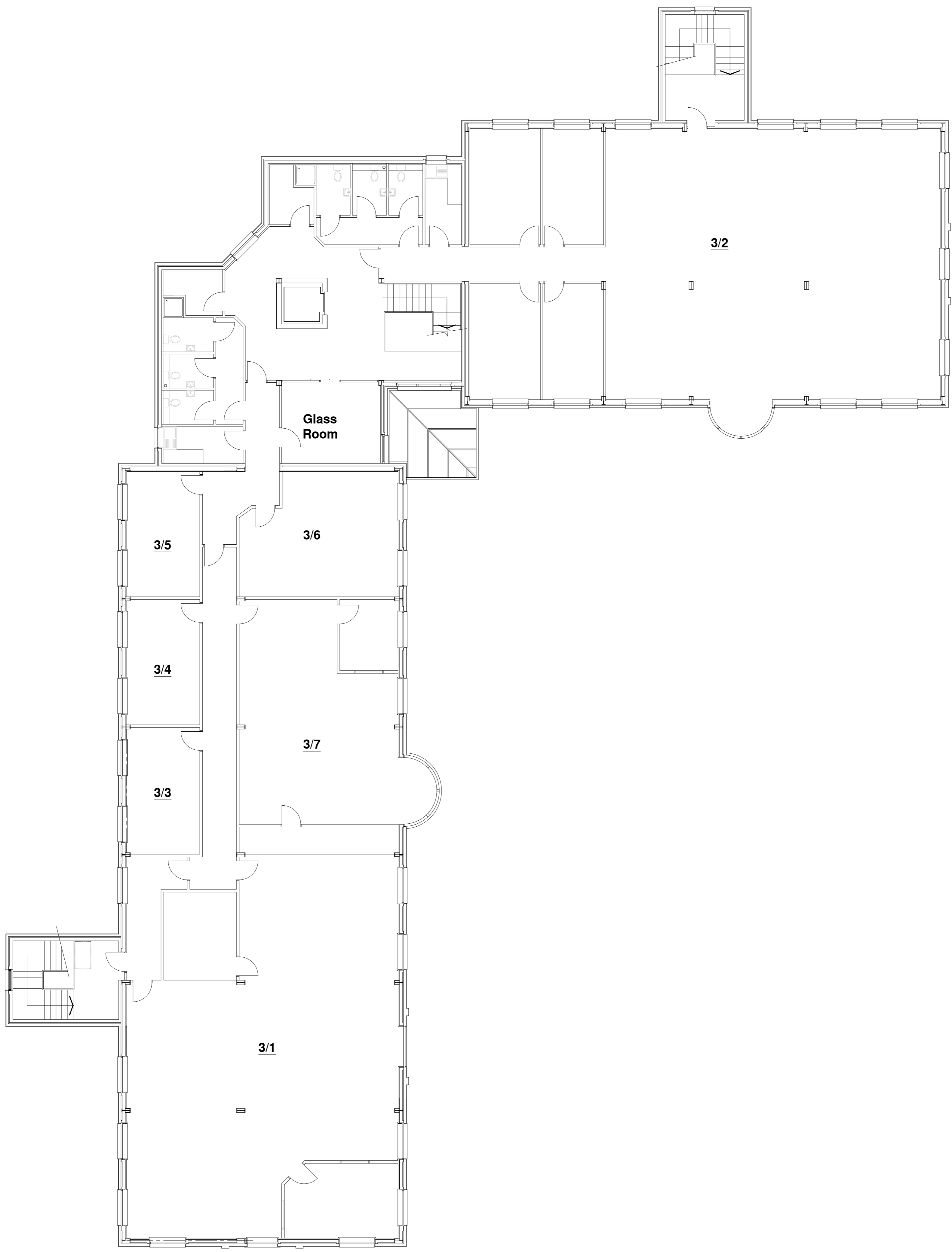
E-CENTRE Second Floor Plan
